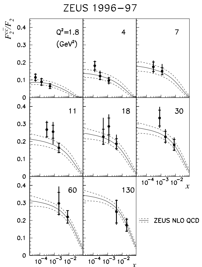
Fig. 9. The ratio of F_2^{cc} to F_2 at Q^2 values between 1.8 and 130 \text{GeV}^2 as a function of x . The ratio is calculated using the F_2^{cc} values measured in this analysis and the ZEUS NLO QCD fit to F_2 [36]. The inner error bars show the statistical uncertainty and the outer ones show the statistical and systematic uncertainties summed in quadrature. The curves correspond to the NLO QCD calculation [7,45] using the result of the ZEUS NLO QCD fit to F_2 [41]. The solid curves correspond to the central values and the dashed curves give the uncertainty due to the parton distributions from the ZEUS NLO fit. Details of this calculation are given in the text. The overall normalization uncertainties arising from the luminosity measurement ( \pm 1.65\% ), the D^{*\pm} and D^0 decay branching ratios, the charm hadronization fraction to D^{*+} ( \pm 9\% ) and the extrapolation uncertainties (see text) are not included
