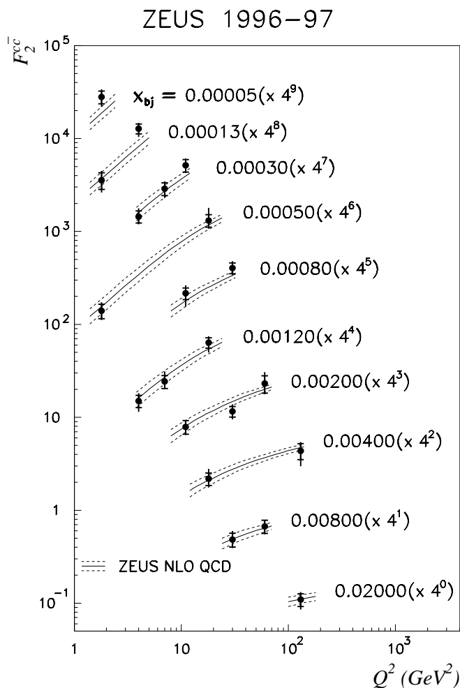
Fig. 8. The measured F_2^{cc} at x values between 0.00005 and 0.02 as a function of Q^2 . The various values of x are indicated to the right of the data points. For clarity of presentation, the F_2^{cc} values have been scaled by the number shown in parentheses next to the x value. The inner error bars show the statistical uncertainty and the outer ones show the statistical and systematic uncertainties summed in quadrature. The curves correspond to the NLO QCD calculation [7,45] using the result of the ZEUS NLO QCD fit to F_2 [41]. The solid curves correspond to the central values and the dashed curves give the uncertainty due to the parton distributions from the ZEUS NLO fit. Details of this calculation are given in the text. The overall normalization uncertainties arising from the luminosity measurement ( \pm 1.65\% ), the D^{*\pm} and D^0 decay branching ratios, the charm hadronization fraction to D^{*+} ( \pm 9\% ) and the extrapolation uncertainties (see text) are not included
