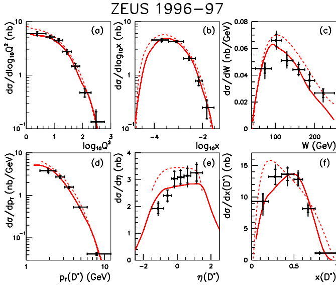
Fig. 6a–f. Differential cross sections for D^{*\pm} production from the K2\pi final state (solid dots) in the accessible Q^2 , y , p_T(D^*) and \eta(D^*) region as functions of a \log_{10} Q^2 , b \log_{10} x , c W , d p_T(D^*) , e \eta(D^*) and f x(D^*) . The inner error bars show the statistical uncertainties while the outer ones show the statistical and systematic uncertainties summed in quadrature. The solid curves show the results of the HVQDIS calculation with RAPGAP-based fragmentation and m_c = 1.4 GeV, while the dashed curves correspond to the BKL results (see text)
