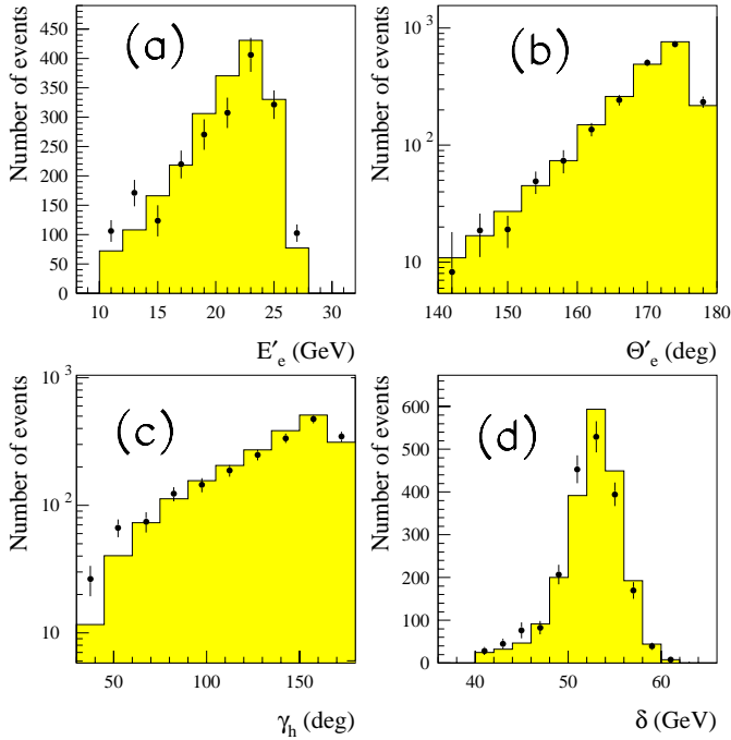
Fig. 3a–d. A comparison of reconstructed DIS quantities at the detector level for the K2\pi data (points) and for the RAPGAP Monte Carlo simulation (shaded histogram): a the scattered positron energy, E'_e , b the scattered positron angle, \theta'_e , c the hadronic angle, \gamma_h and d \delta \equiv \Sigma_i(E_i - p_{z,i})
