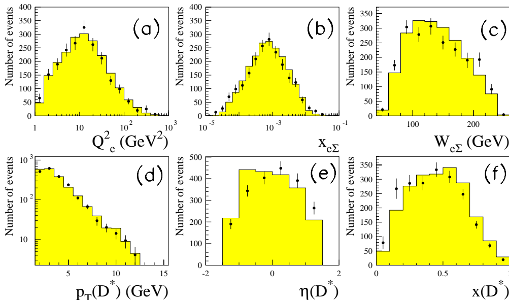
Fig. 4a–f. A comparison of the reconstructed DIS kinematic distributions at the detector level for the K2\pi data (points) and for the RAPGAP Monte Carlo simulation (shaded histogram): a Q_e^2 , b Bjorken- x , x_{e\Sigma} and c the total hadronic center-of-mass energy, W_{e\Sigma} . The remaining plots show a comparison of the reconstructed D^{*\pm} -related quantities at the detector level for data and for the RAPGAP Monte Carlo simulation: d p_T(D^*) , e \eta(D^*) and f x(D^*)
