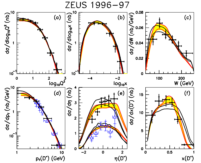
Fig. 5a–f. Differential cross sections for D^{*\pm} production from the K2\pi final state (solid dots) in the Q^2 , y , p_T(D^*) and \eta(D^*) kinematic region as functions of a \log_{10} Q^2 , b \log_{10} x , c W , d p_T(D^*) , e \eta(D^*) and f x(D^*) . The inner error bars show the statistical uncertainties while the outer ones show the statistical and systematic uncertainties summed in quadrature. The results from the K4\pi channel (open triangles) are also shown in the p_T(D^*) d and \eta(D^*) e plots. The data are compared with the NLO QCD calculation as implemented in HVQDIS using the ZEUS NLO pdf's. The open band corresponds to the standard Peterson fragmentation function with the parameter \epsilon = 0.035 . For the shaded band, the Peterson fragmentation was replaced by that extracted from RAPGAP (see the text for details). The boundaries of the bands correspond to charm mass variations between 1.3 (upper curve) and 1.5 \text{GeV} (lower curve). In a and b , the open band is indistinguishable from the shaded band
