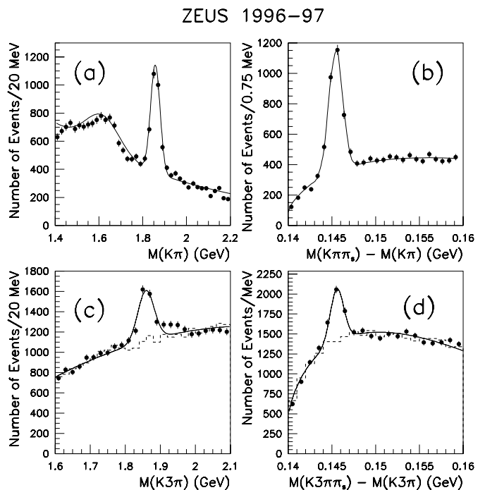
Fig. 2a–d. ZEUS data in the kinematic region 1 < Q^2 < 600 \text{GeV}^2 and 0.02 < y < 0.7 : a M(D^0) = M(K\pi) and b \Delta M = M(K\pi\pi_s) - M(K\pi) for the K2\pi final state. The data are shown in the same kinematic region for the K4\pi final state in c M(D^0) = M(K3\pi) and d \Delta M = M(K3\pi\pi_s) - M(K3\pi) . The events in a and c are those for which 143 < \Delta M < 148 MeV. Similarly, b and d are shown for events in the M(D^0) signal region: 1.80-1.92 (1.81-1.91) GeV for the K2\pi ( K4\pi ) channel. The solid curves are the results of the fits described in the text. The dashed histograms in c and d represent the background distributions obtained by restricting the sample to side-bands from the \Delta M and M(D^0) distributions, respectively
