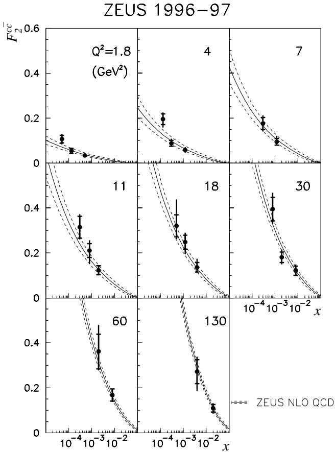
Fig. 7. The measured F_2^{c\bar{c}} at Q^2 values between 1.8 and 130 \text{GeV}^2 as a function of x . The inner error bars show the statistical uncertainty and the outer ones show the statistical and experimental systematic uncertainties summed in quadrature. The curves correspond to the NLO QCD calculation [7, 45] using the result of the ZEUS NLO QCD fit to F_2 [41]. The solid curves correspond to the central values and the dashed curves give the uncertainty due to the parton distributions from the ZEUS NLO fit. The overall normalization uncertainties arising from the luminosity measurement ( \pm 1.65\% ), the D^{*\pm} and D^0 decay branching ratios, the charm hadronization fraction to D^{*+} ( \pm 9\% ) and the extrapolation uncertainties (see text) are not included
