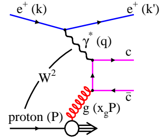
Fig. 1. Diagram of the boson-gluon-fusion process in e^+p collisions
